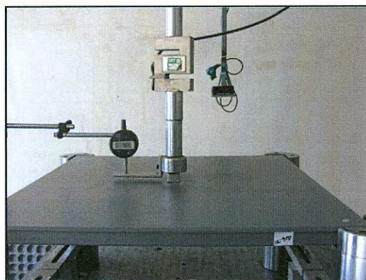
PHOTO 2: Images of UNITILE USF LFW 30 0800 (Corner Lock) while Testing
