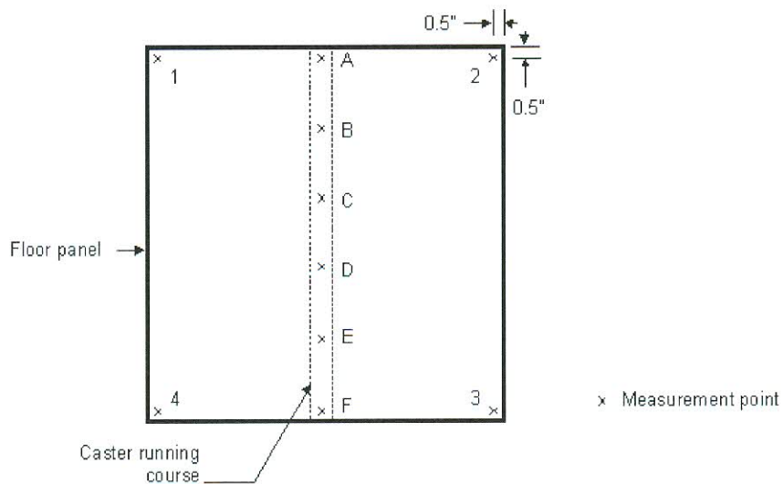
Figure 1: Position of Measurement (Rolling Load)
