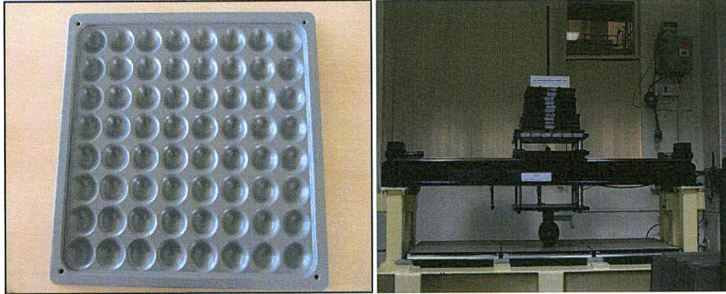
PHOTO 1: Images of UNITILE UFP 30 0800 (Corner Lock) before /while Testing
