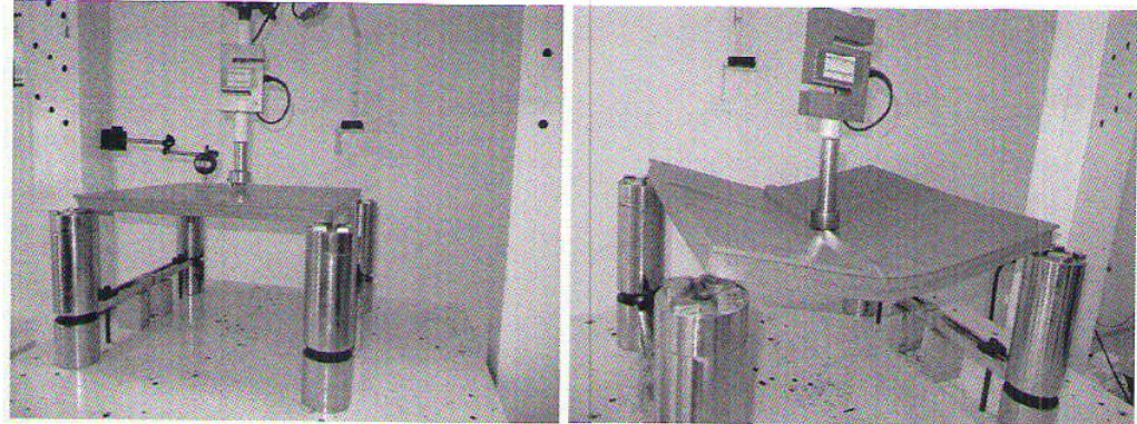
UNITILE UFP 30 1650 Bare - TEST UNDER PROGRESS
