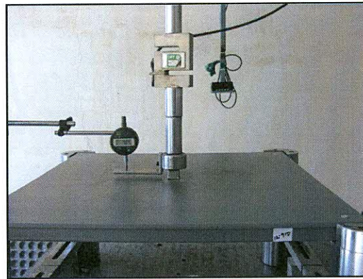
PHOTO 2: Images of UNITILE UFP 35 1000 (Corner Lock) while Testing
