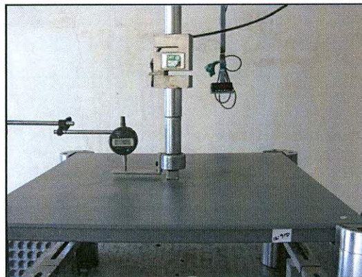
PHOTO 2: Images of UNITILE UFP 30 0800 (Corner Lock) while Testing
