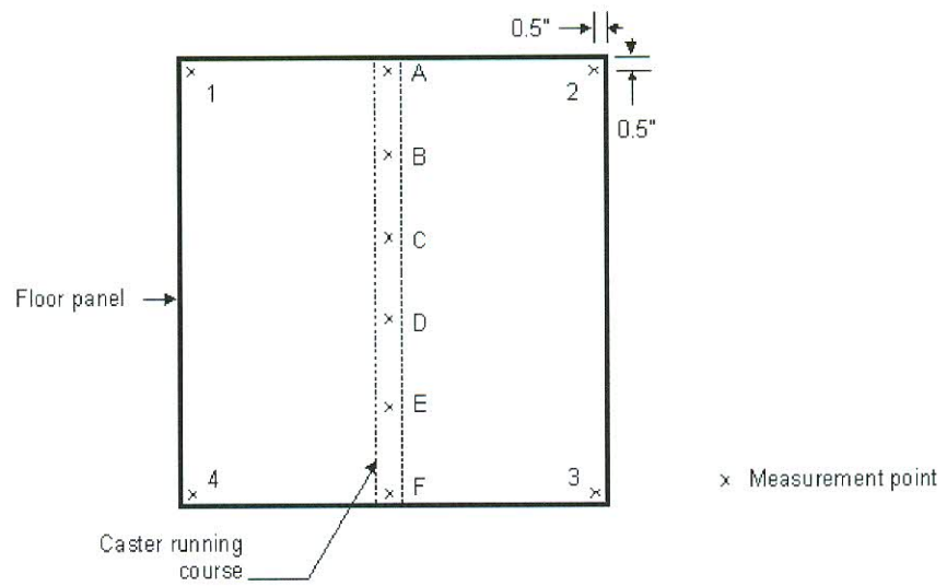
Figure 1: Position of Measurement (Rolling Load)
